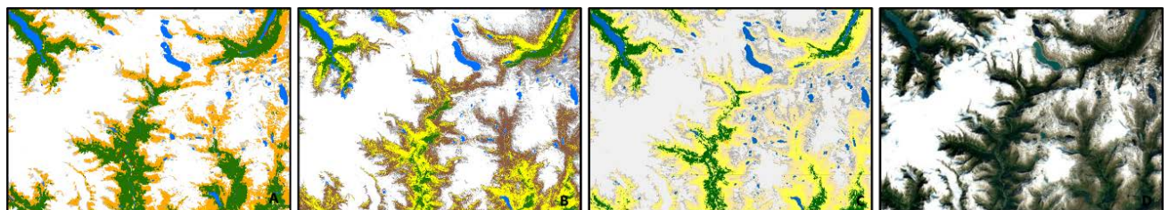
Figure 11 Comparison of Esri 2020 landcover (A), FROM-GLC10 (B), WorldCover 2020 (C), and Google Earth (D) for a snow/ice area in Jostedalsgreen National Park, Norway. (Coordinates: 61°43'59.9"N 7°18'19.3"E), see Figure 5 for legend
